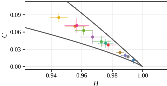
Shannon, D = 5 (RSAM, Feb)
