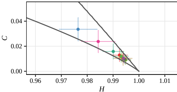
Shannon, D = 5 (Displacement, Jun)
