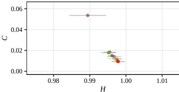
Tsallis, D = 5 (Displacement, Aug)
