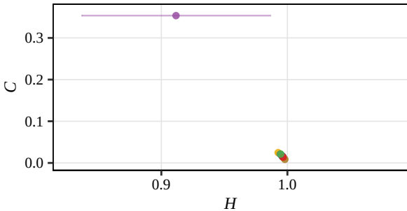
Tsallis, D = 5 (Displacement, Dec)
