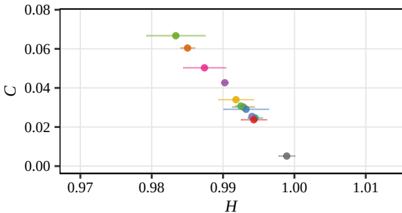
Tsallis, D = 5 (RSAM, May)
