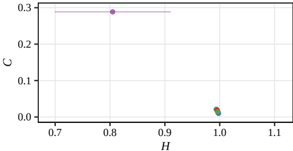
Tsallis, D = 5 (Displacement, Sep)
