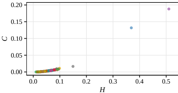
Fisher, D = 5 (RSAM)
