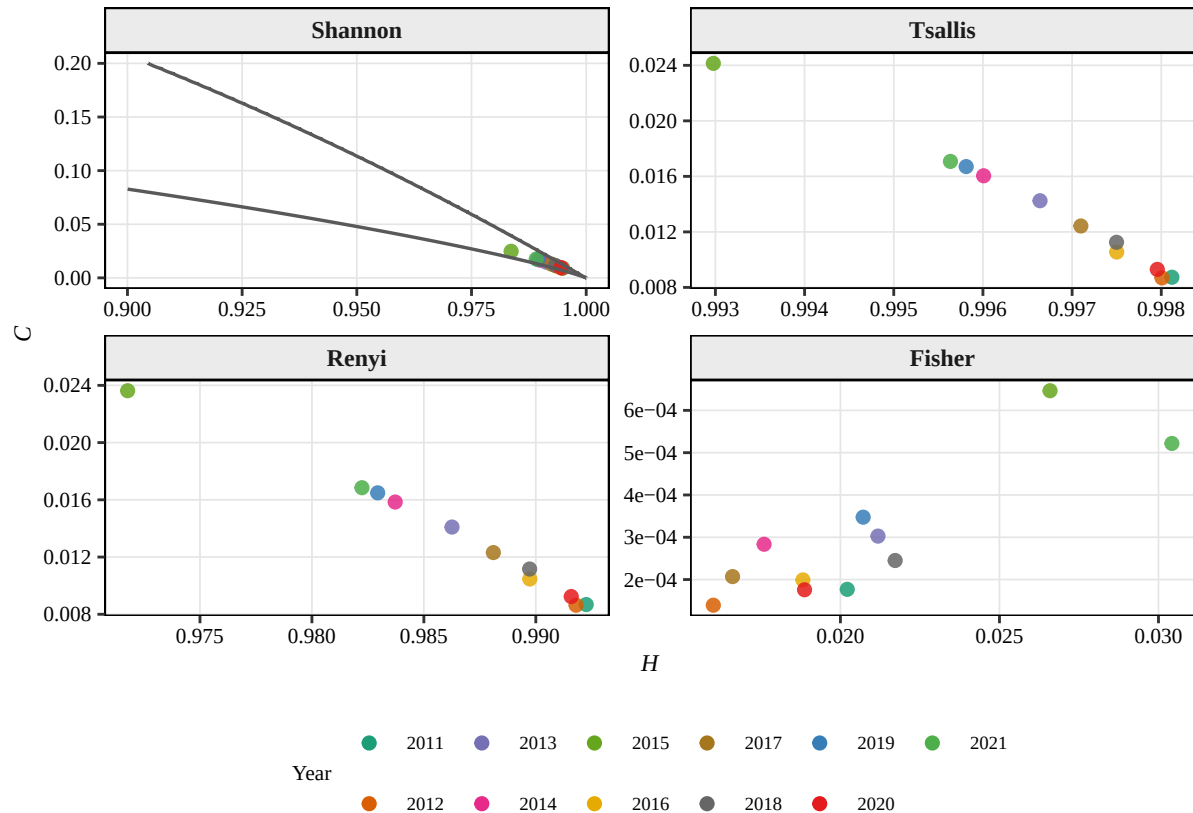
May H \times C planes, D = 5 (Displacement)
