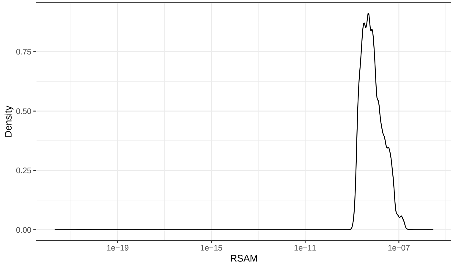
Density plot of RSAM, 2011--2022
