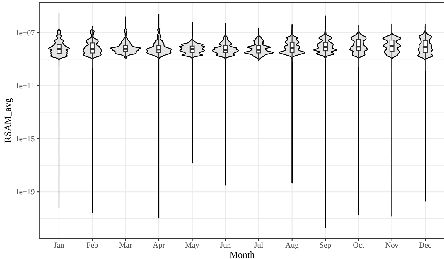
Monthly distribution of RSAM Average, 2011–2022
