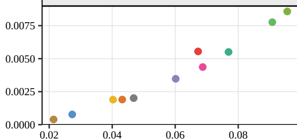
Fisher
