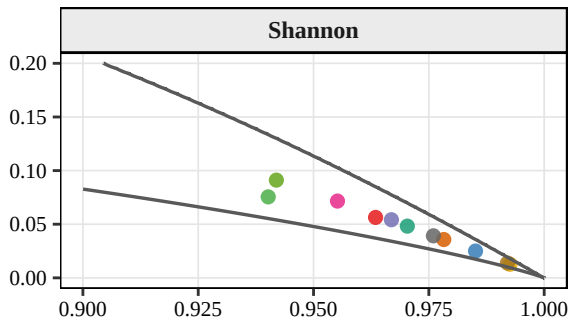
Oct H \times C planes, D = 5 (RSAM)
