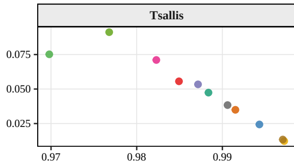
Oct H \times C planes, D = 5 (RSAM)
