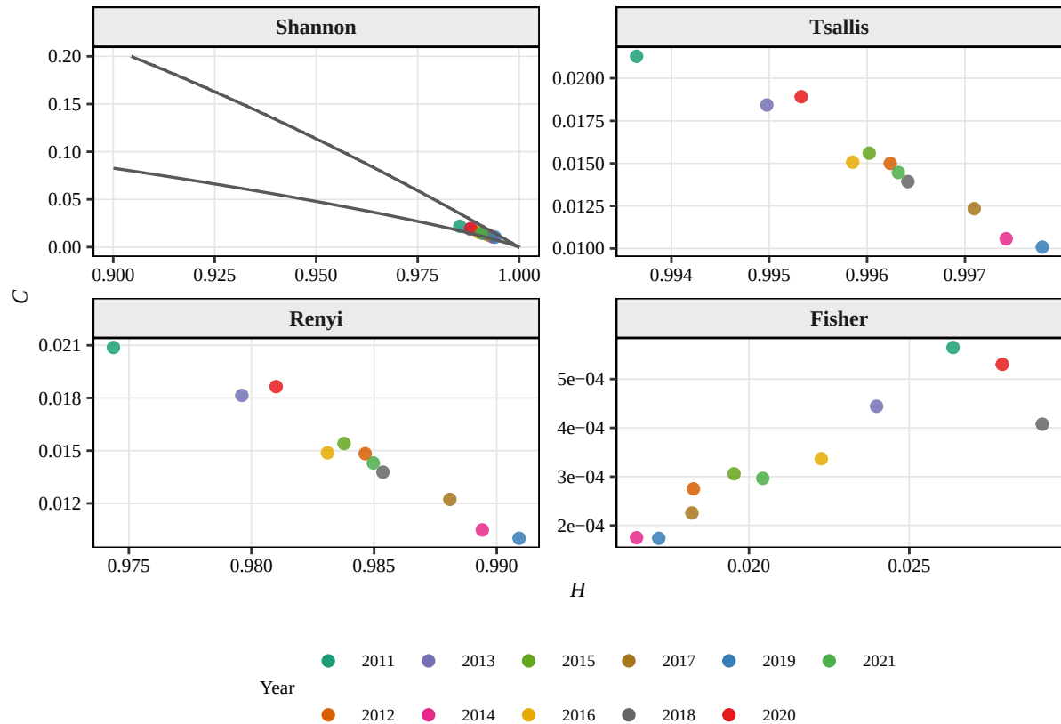
Sep H \times C planes, D = 5 (Displacement)
