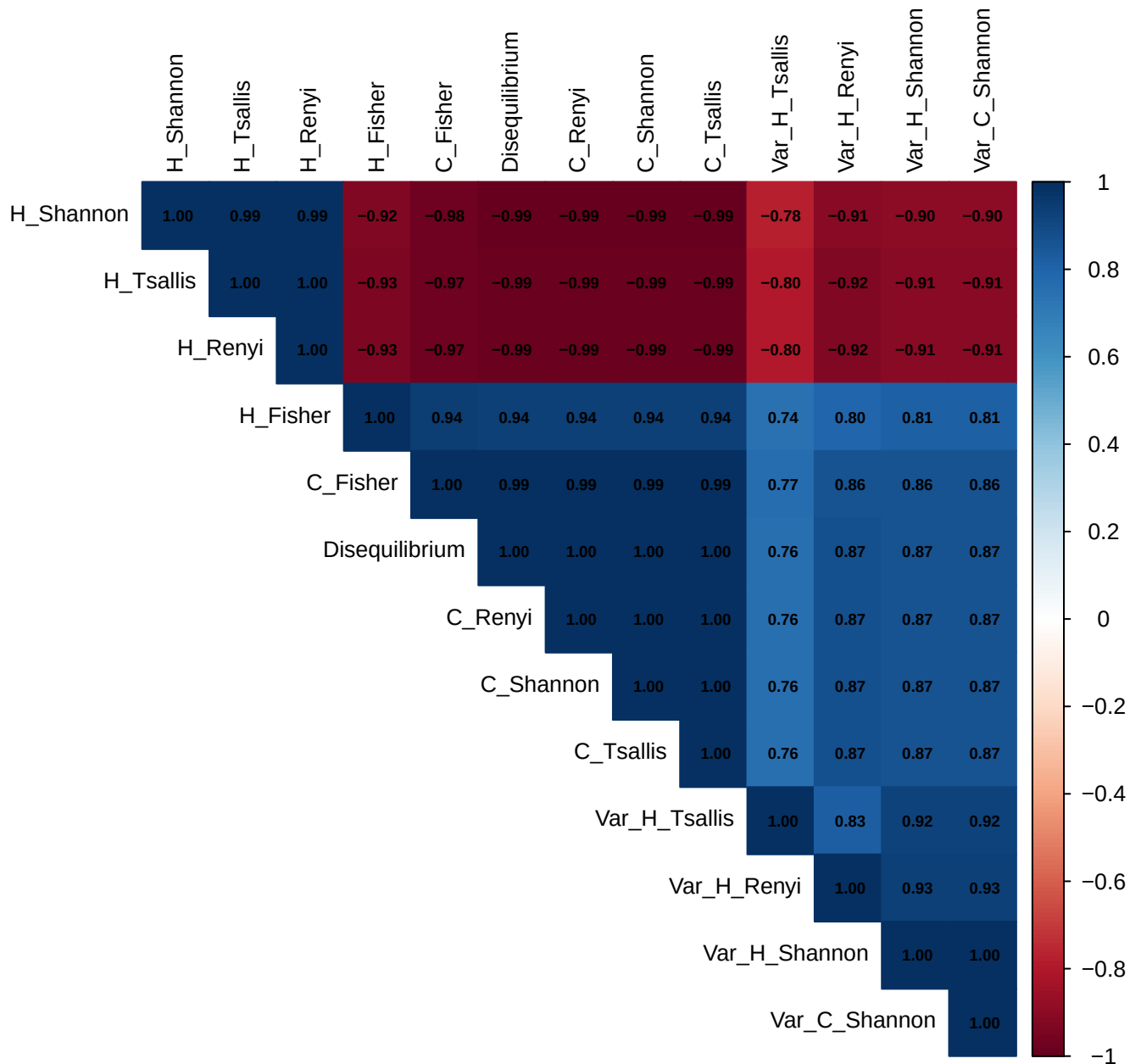
RSAM feature correlation: 2013
