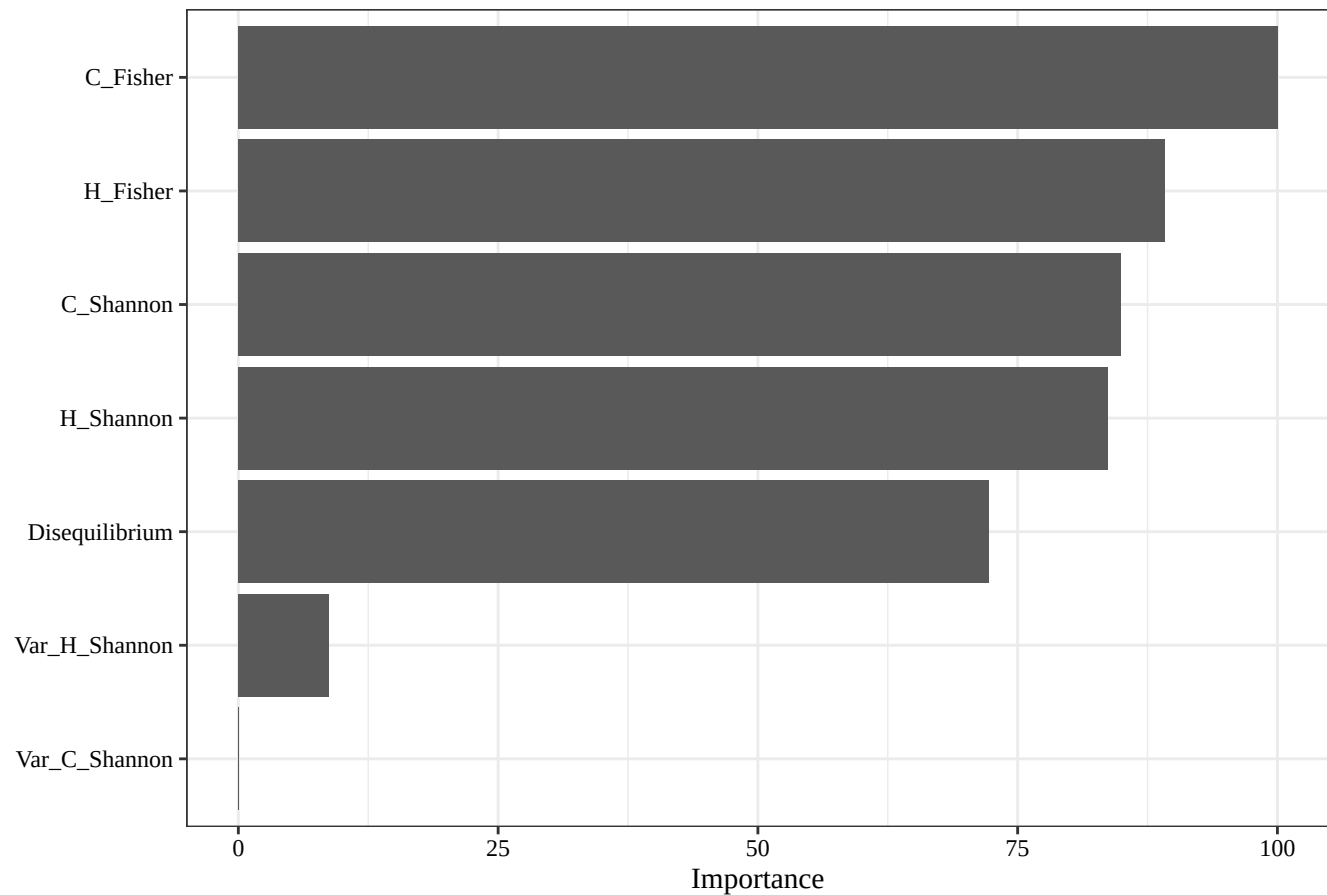
Random Forest feature importance: Dec
