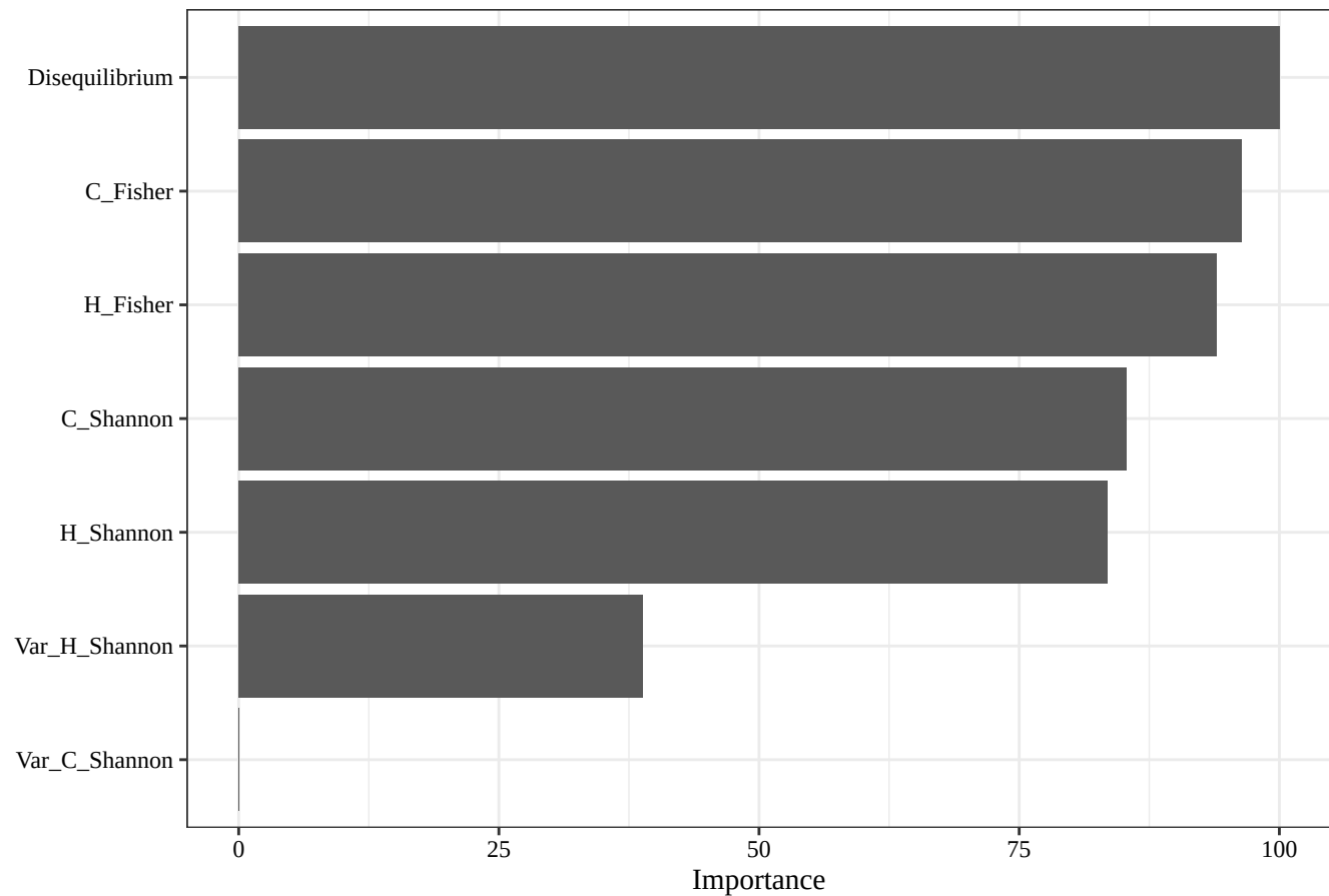
Random Forest feature importance: Feb
