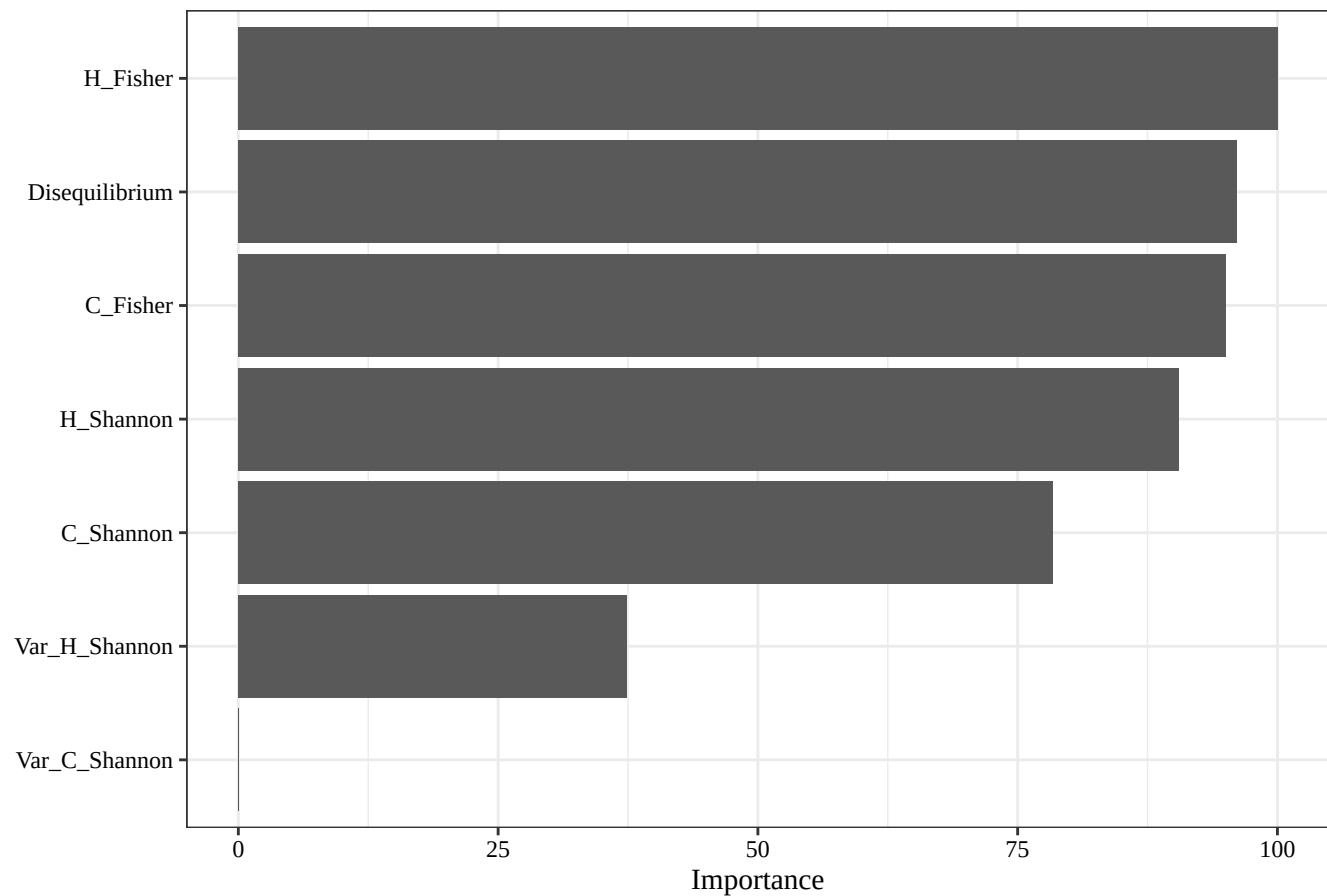
Random Forest feature importance: May
