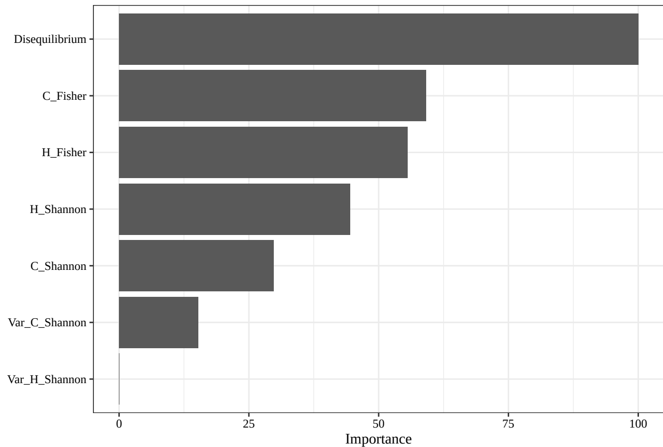
Random Forest feature importance: Oct
