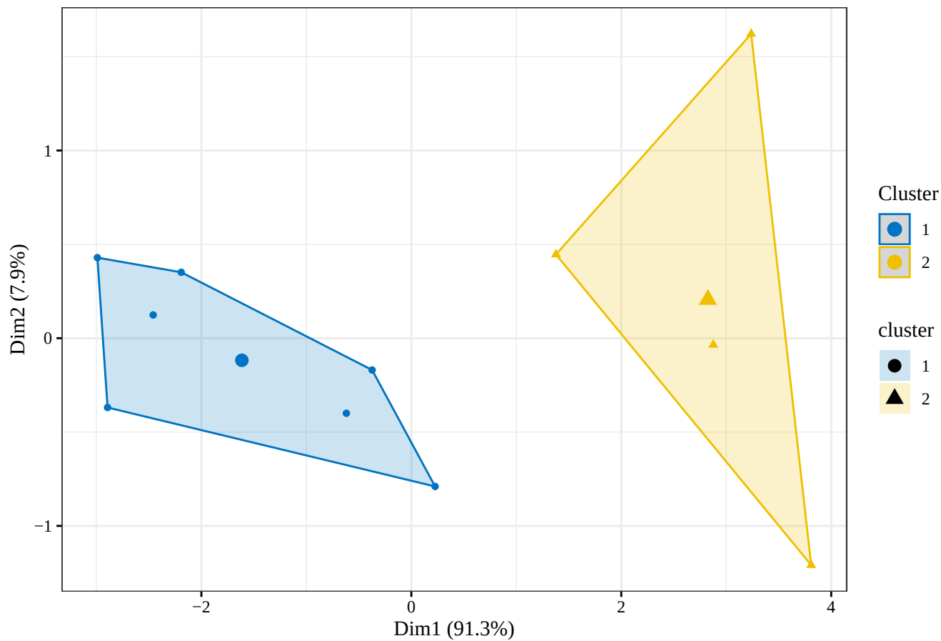
RSAM K-means clusters: Feb , k = 2
