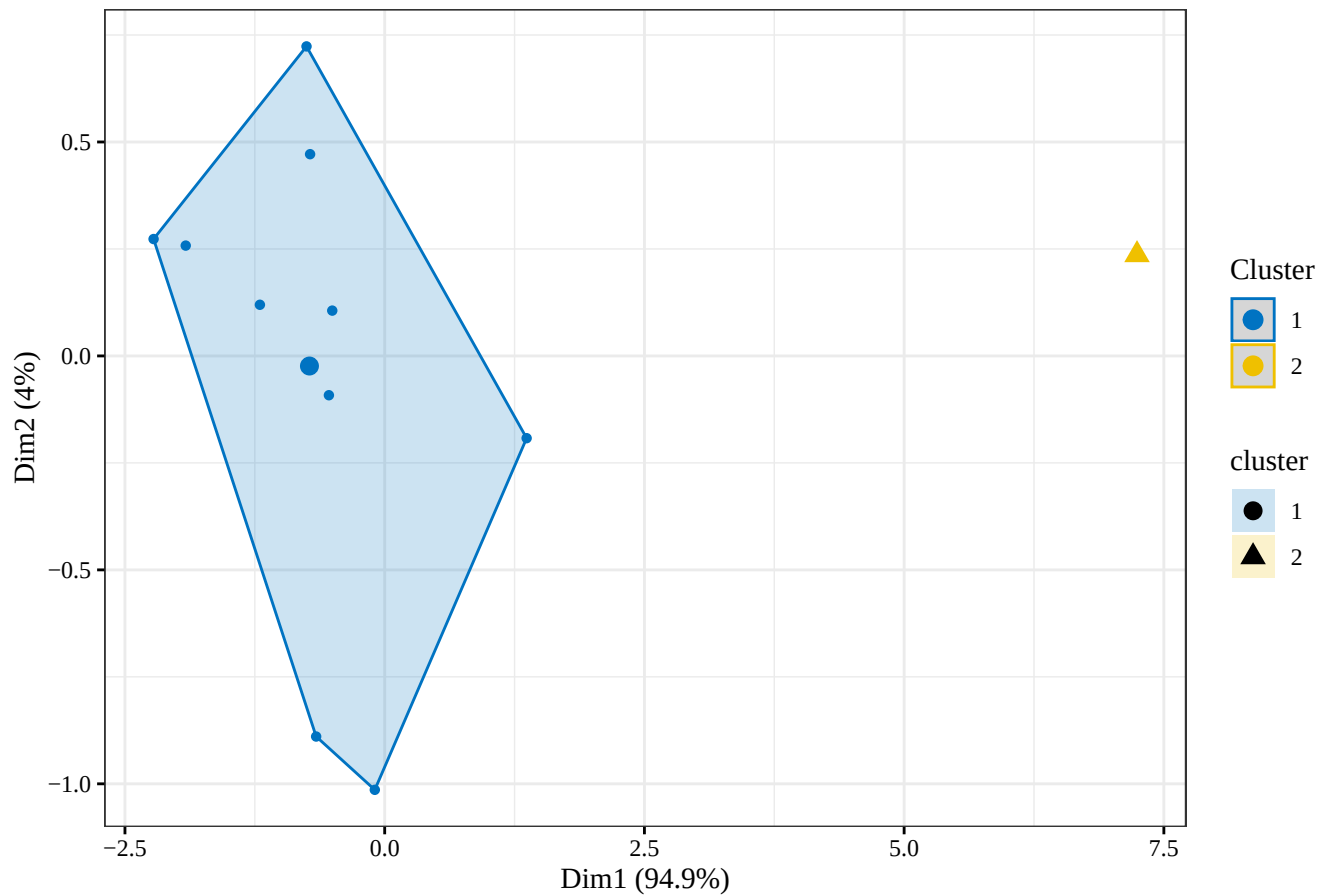
RSAM K-means clusters: Jun , k = 2
