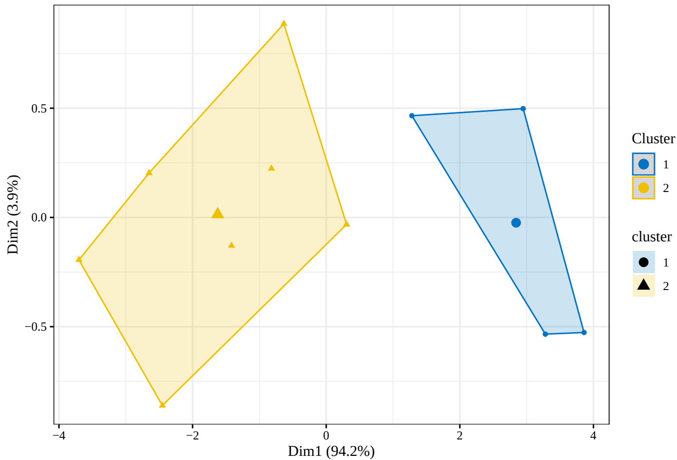
RSAM K-means clusters: Mar , k = 2
