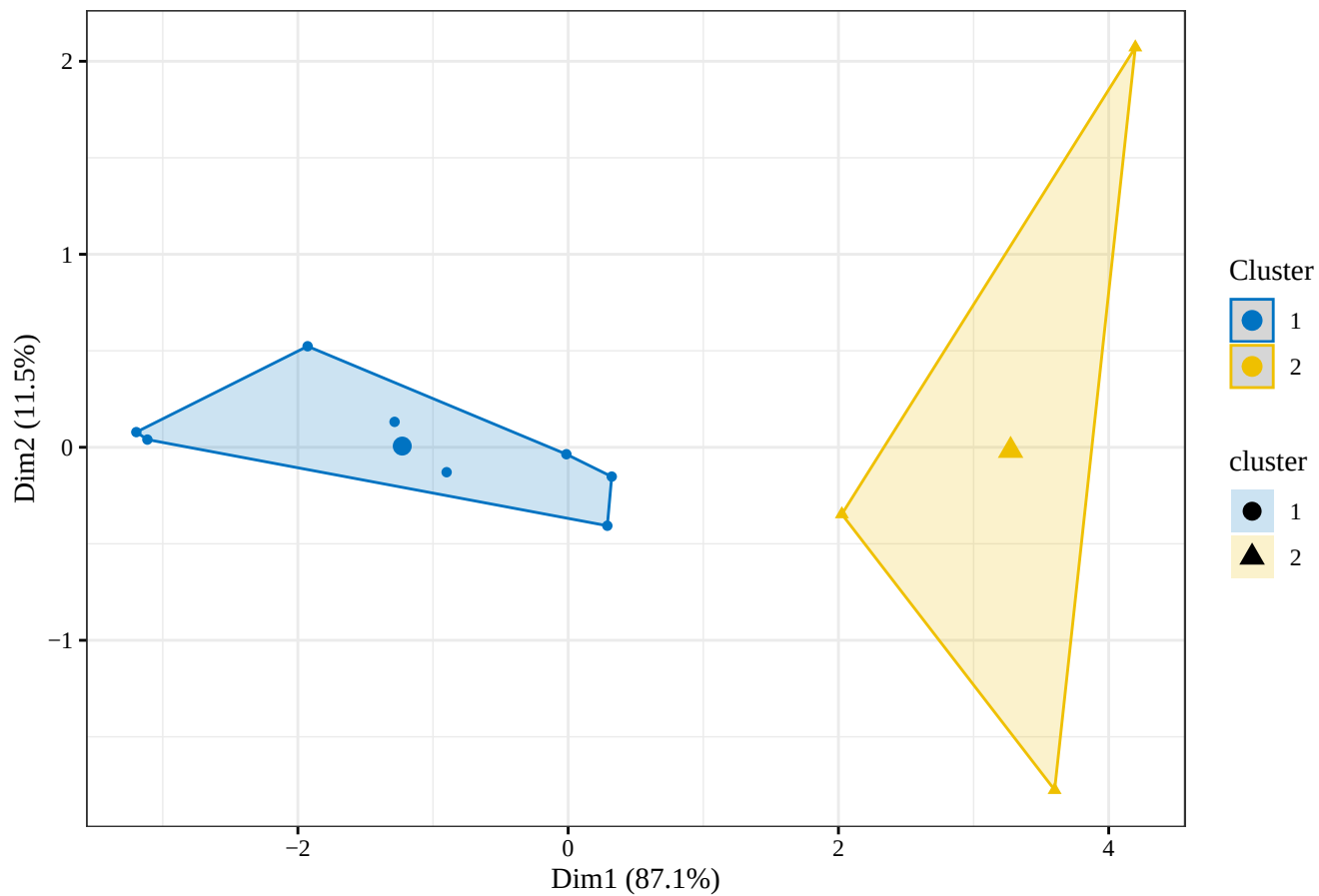
RSAM K-means clusters: Oct , k = 2
