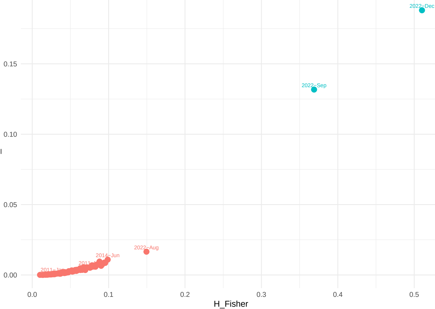
RSAM Monthly – Fisher HC plane
