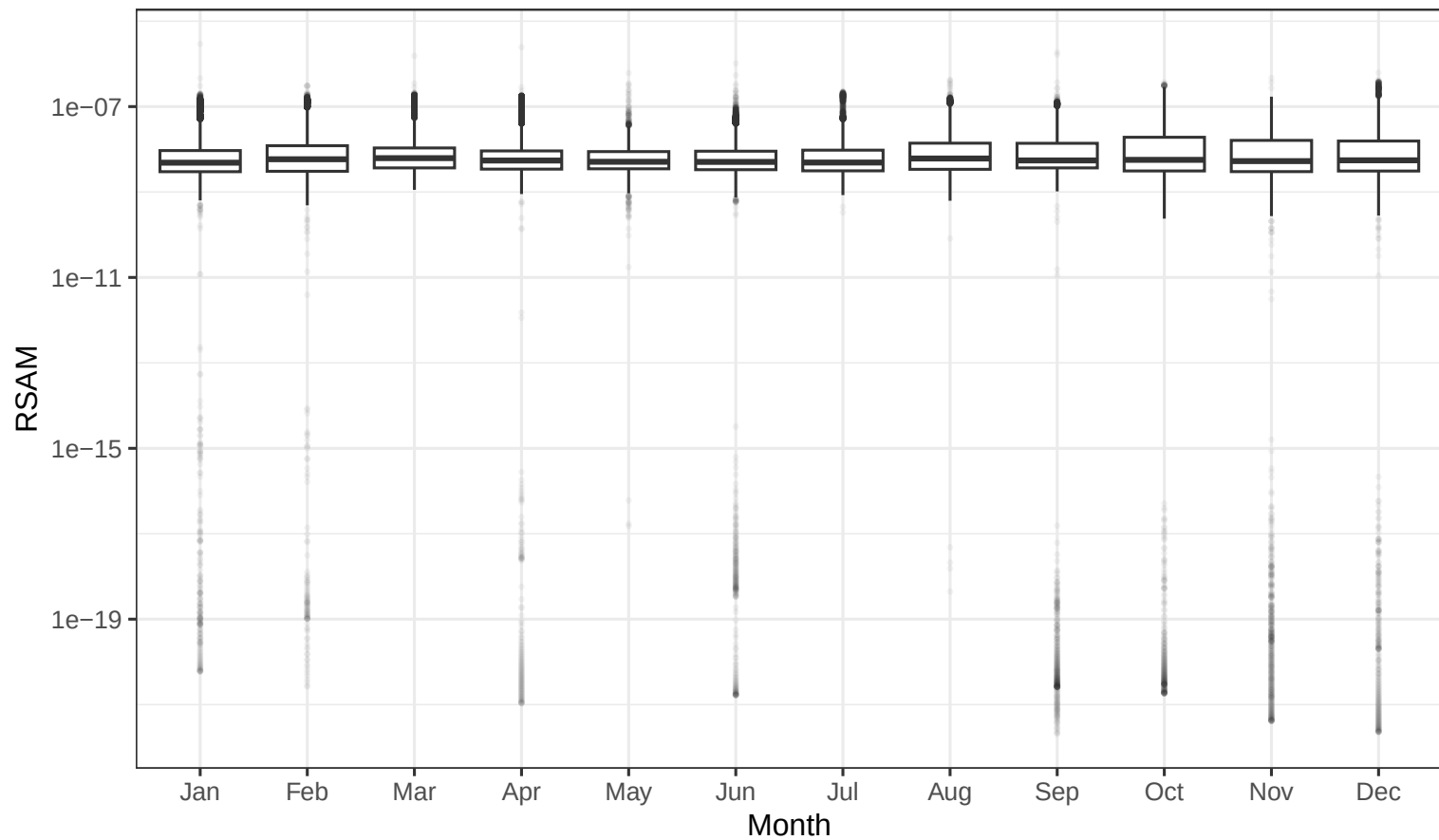
Monthly distribution of RSAM, 2007–2022
