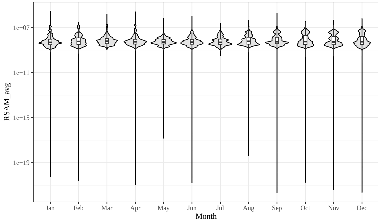
Monthly distribution of RSAM Average, 2007–2022
