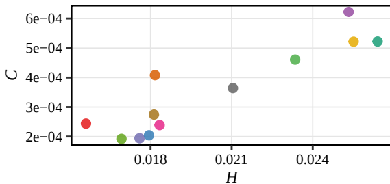
Fisher
