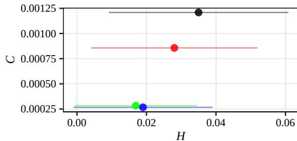
Fisher
