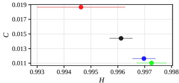
Fisher
