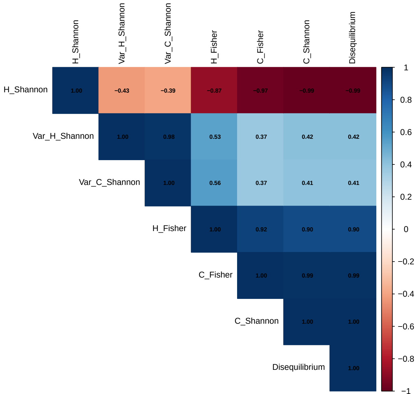
RSAM feature correlation: 2009
