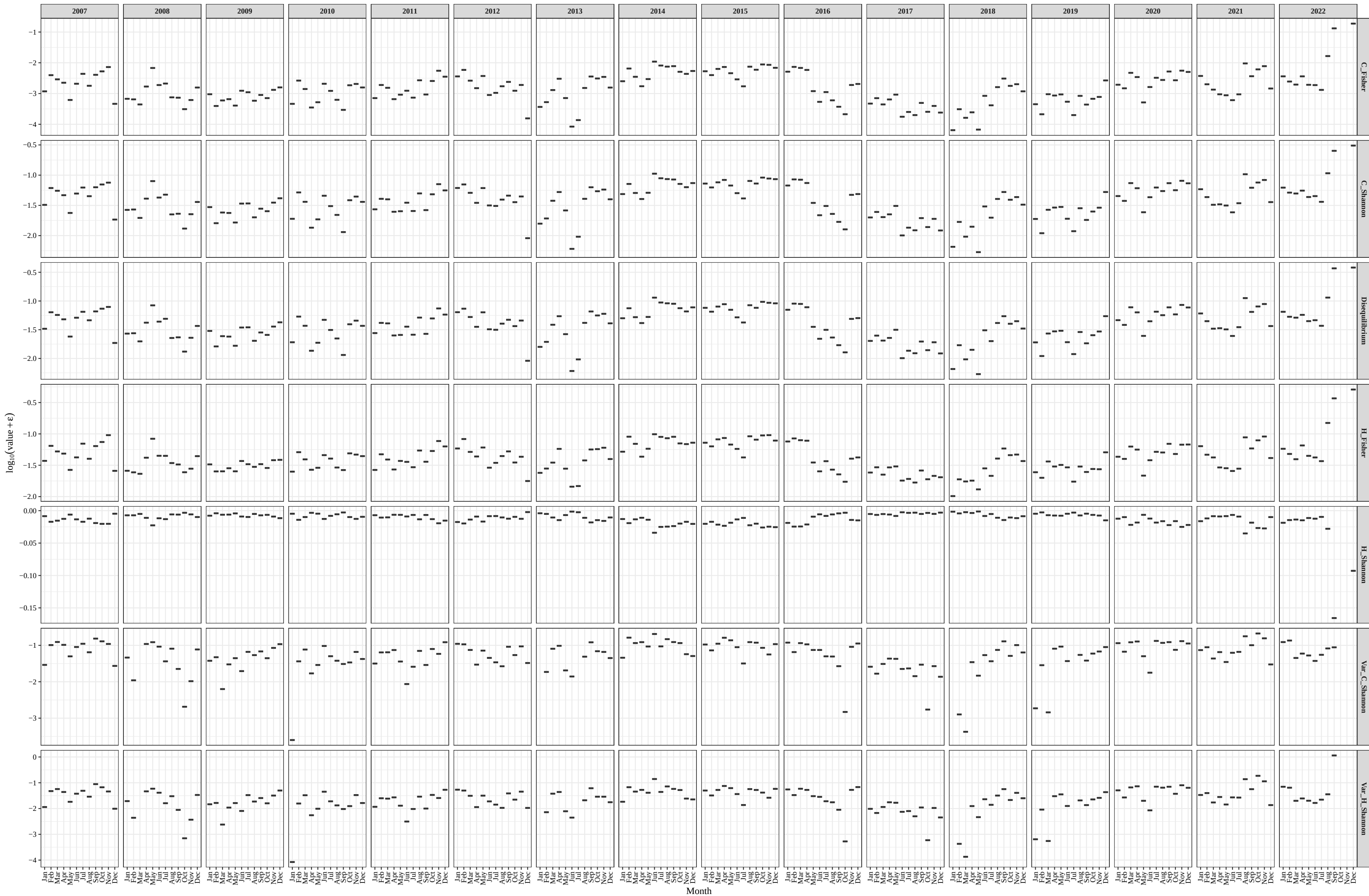
RSAM ordinal-pattern features by month within each year
