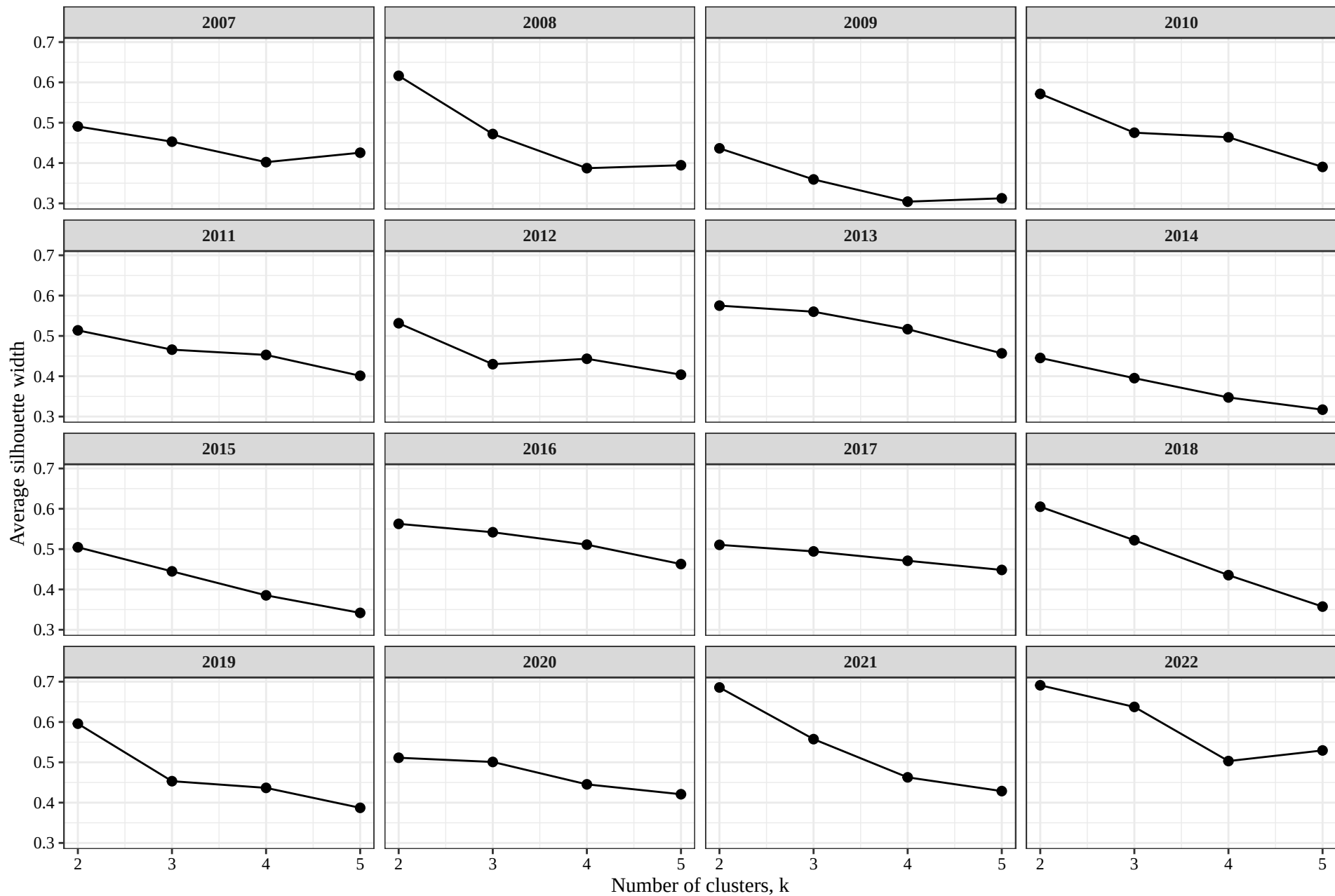
K-means silhouette evaluation by year
