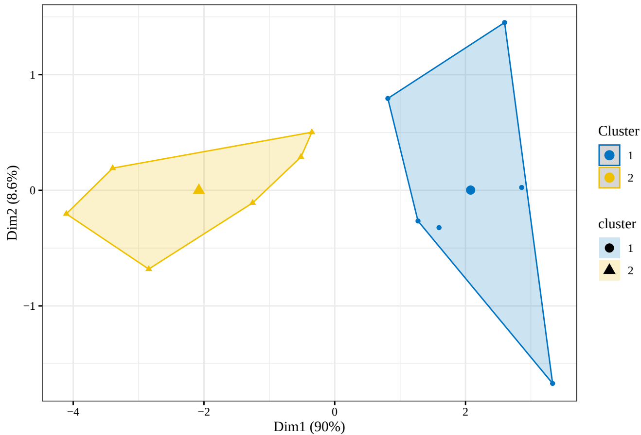
RSAM K-means clusters: 2007 , k = 2
