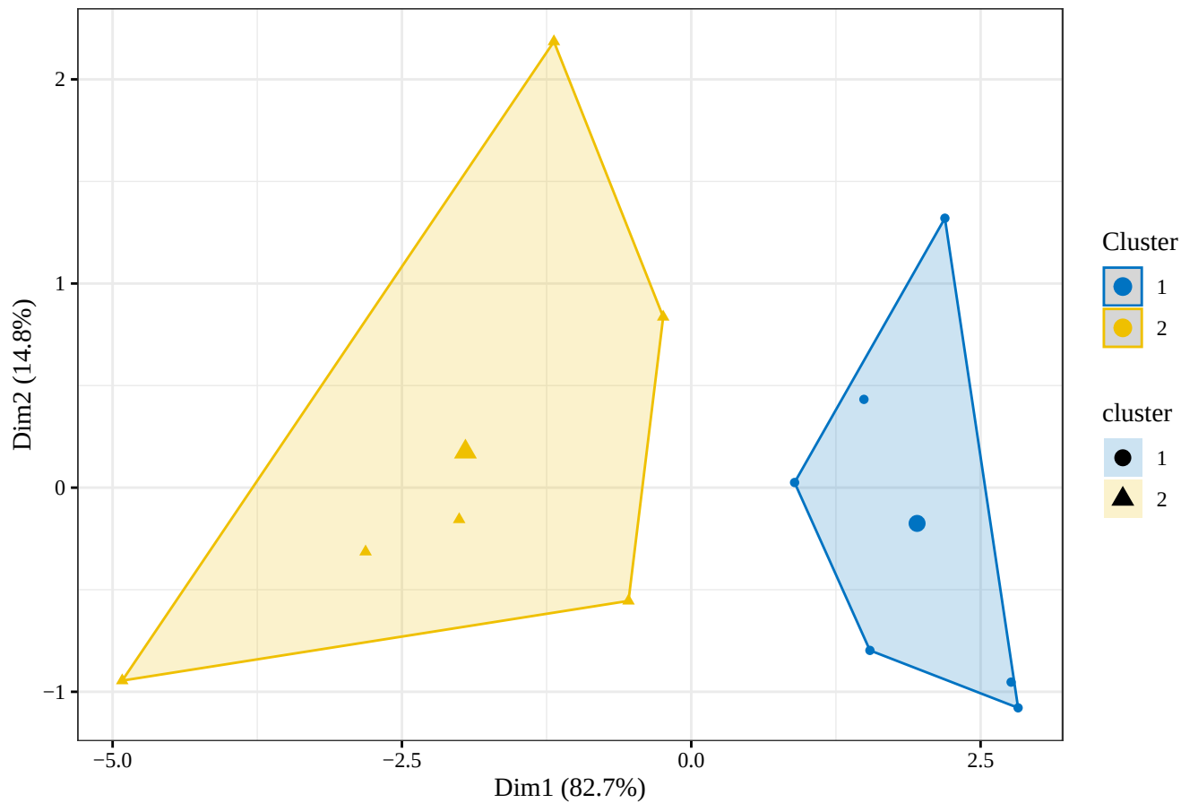
RSAM K-means clusters: 2009 , k = 2
