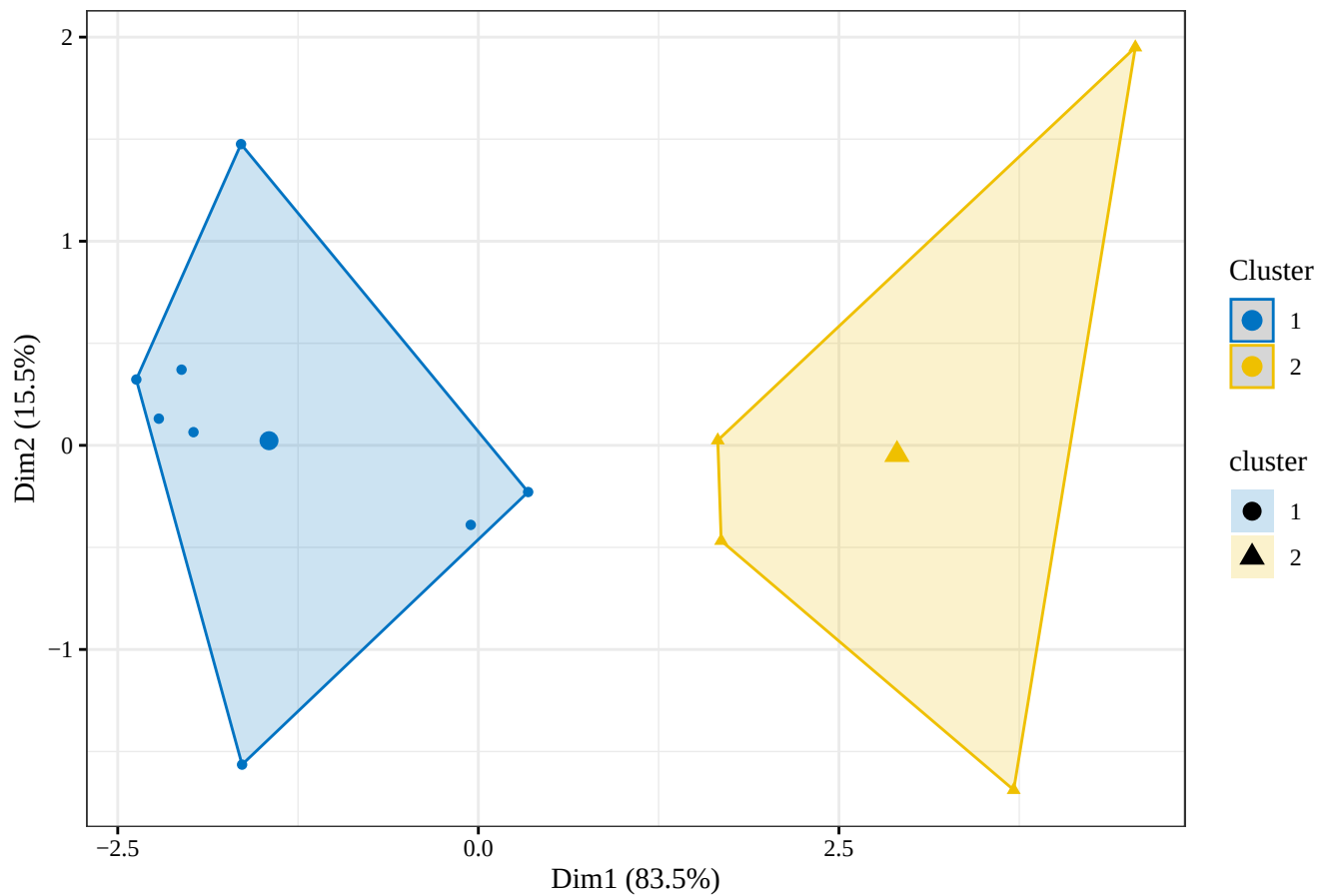
RSAM K-means clusters: 2011 , k = 2
