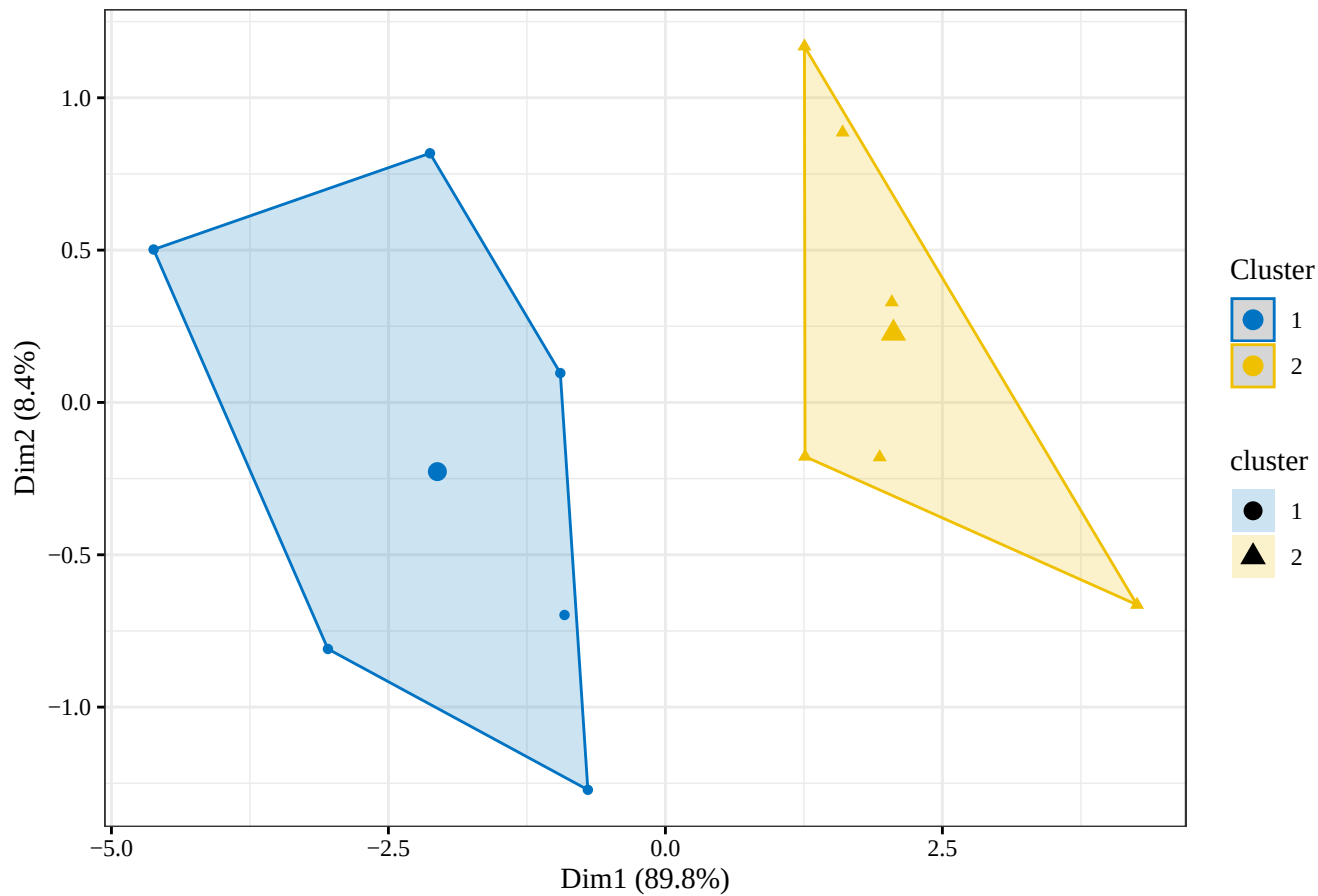
RSAM K-means clusters: 2012 , k = 2
