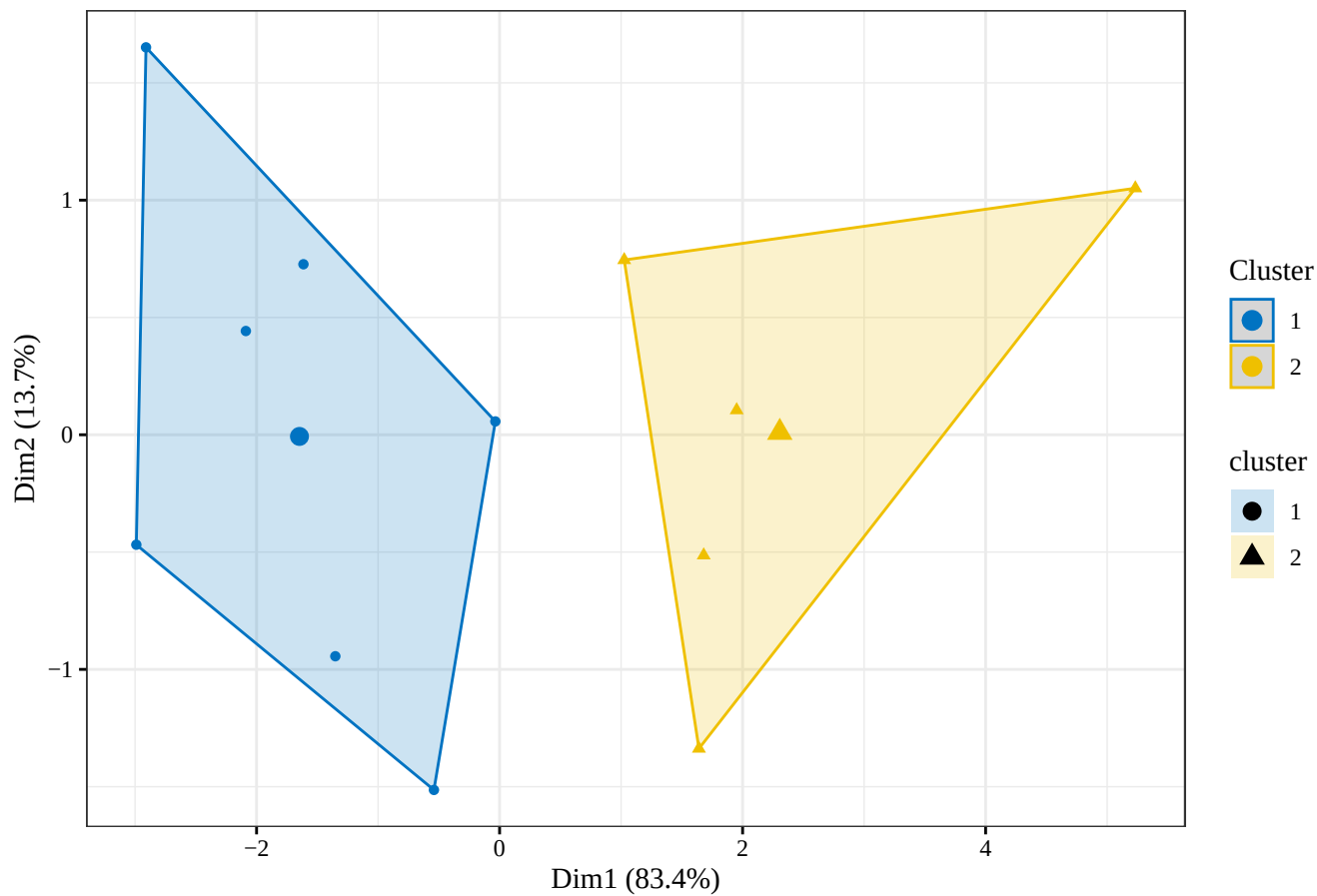
RSAM K-means clusters: 2014 , k = 2
