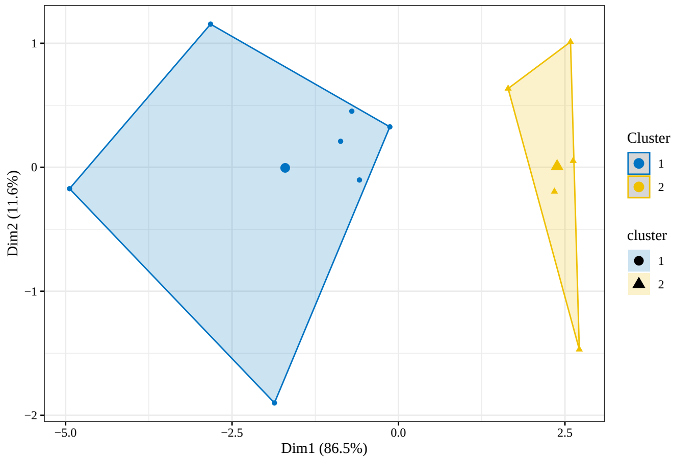
RSAM K-means clusters: 2017 , k = 2
