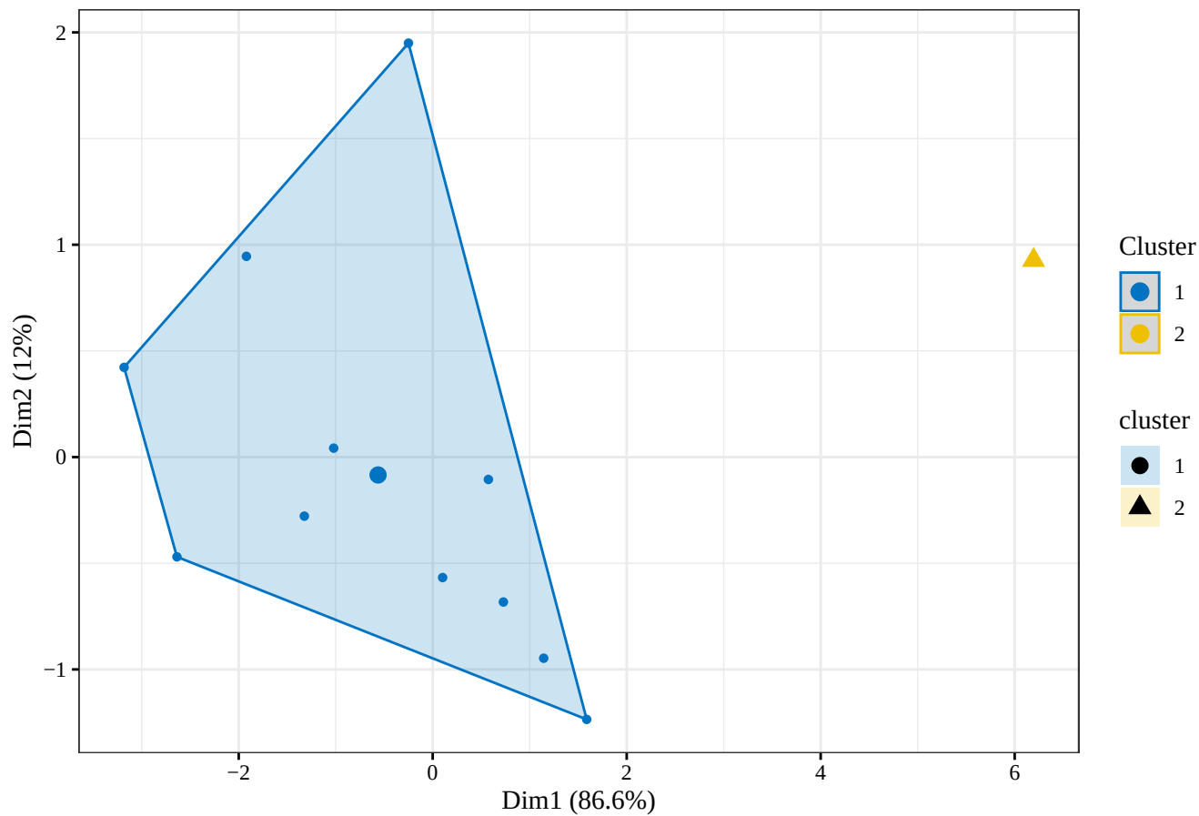
RSAM K-means clusters: 2019 , k = 2
