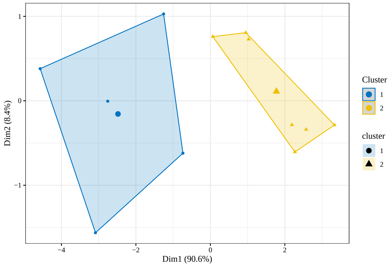
RSAM K-means clusters: 2020 , k = 2
