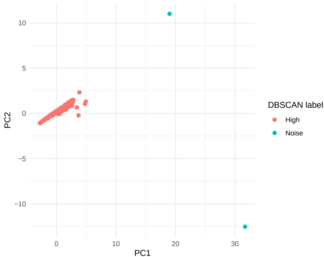
RSAM: DBSCAN (eps=3.31, minPts=14)
