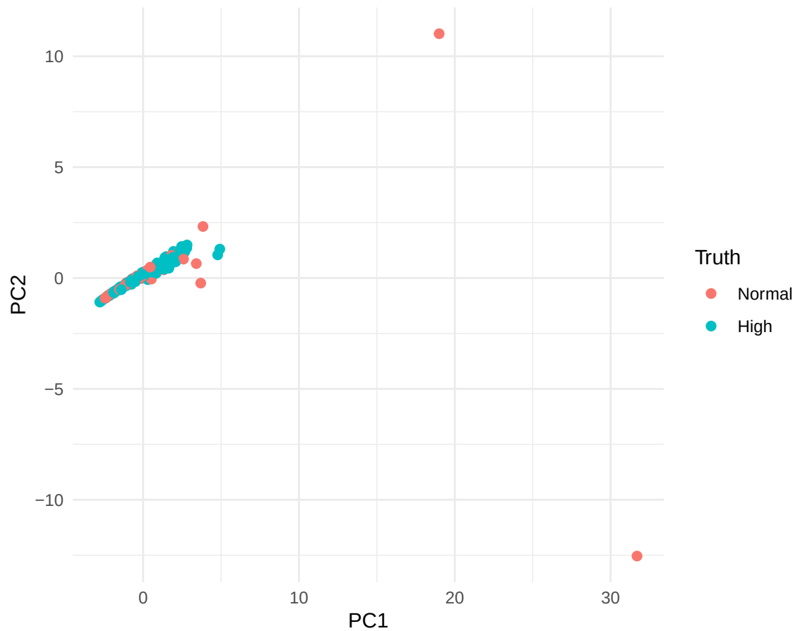
RSAM: Known eruption ground truth
