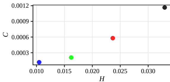
Fisher
