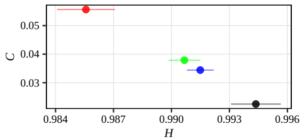
Fisher
