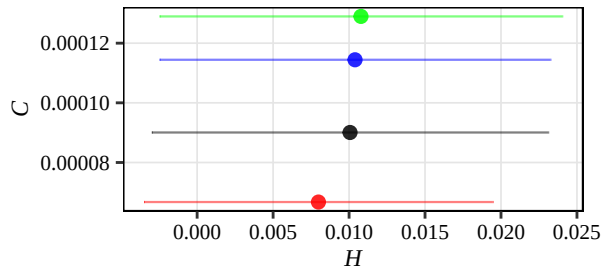
Fisher
