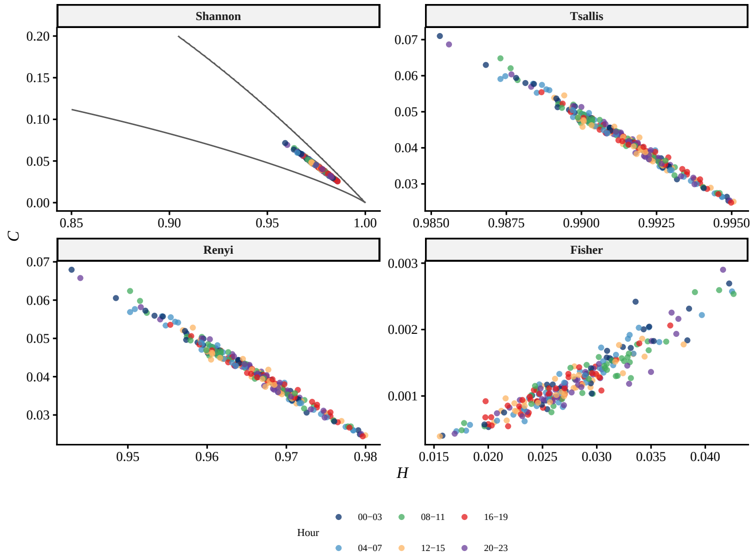
Aug H \times C planes by measure, D = 5 (WIZ, hourly, 2019)
