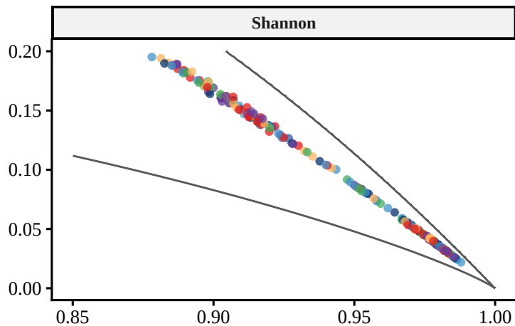
Nov H \times C planes by measure, D = 5 (WIZ, hourly, 2019)
