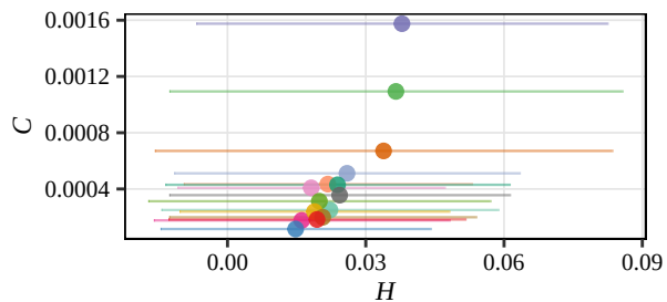
Fisher
