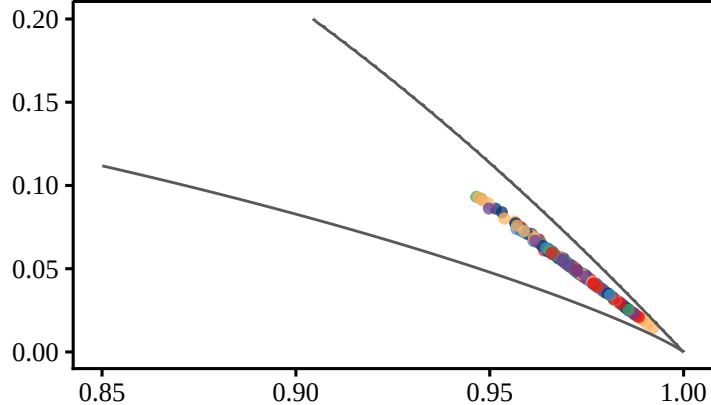
Oct H \times C planes by measure, D = 5 (WIZ, hourly, 2019)
