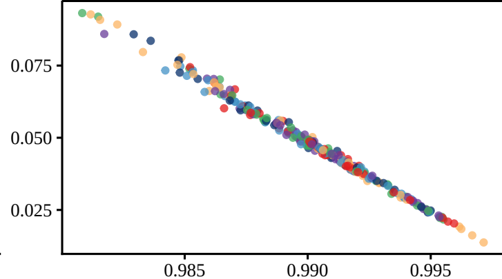
Oct H \times C planes by measure, D = 5 (WIZ, hourly, 2019)
