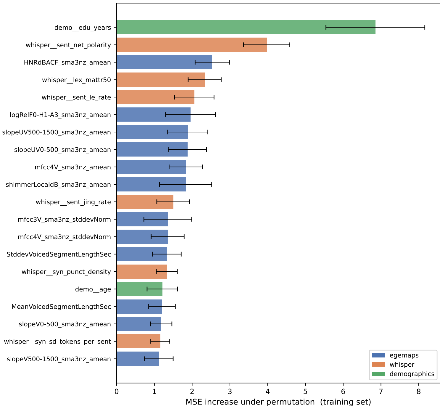
Permutation importance — top 20 EN-selected features
