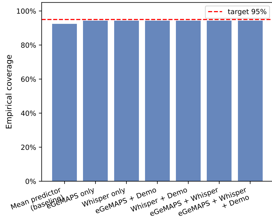
PI coverage (target = 95%)
