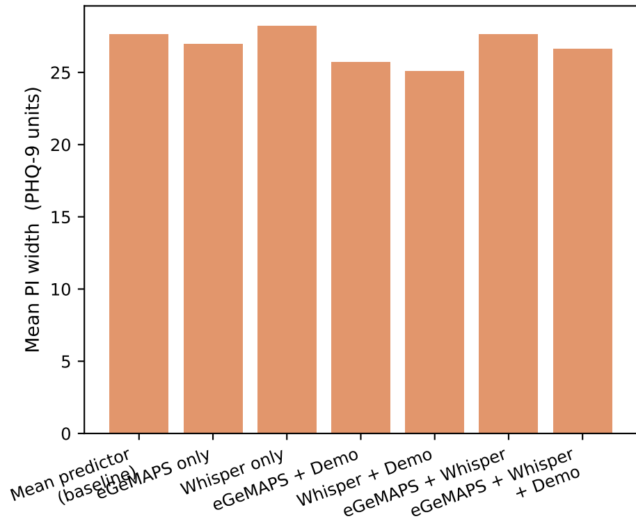
PI mean width (lower = tighter)
